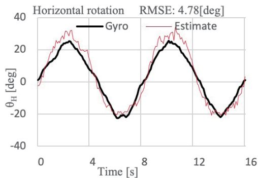
Fig. 13. (Color online) Experimental results of horizontal rotation.
