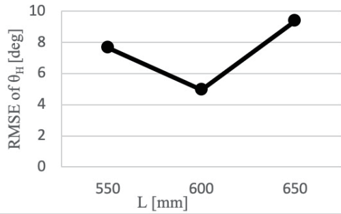
Fig. 11. RMSE values of horizontal rotation for different lengths.
