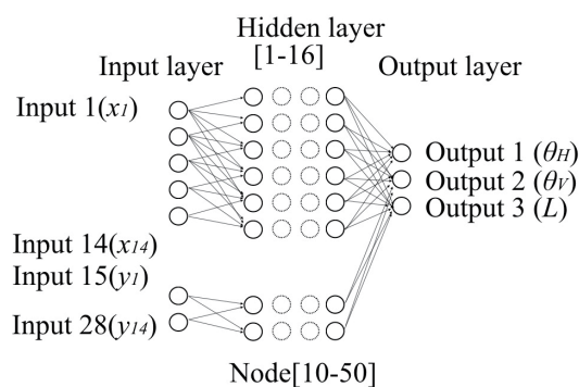
Fig. 3. Structure of deep learning.
