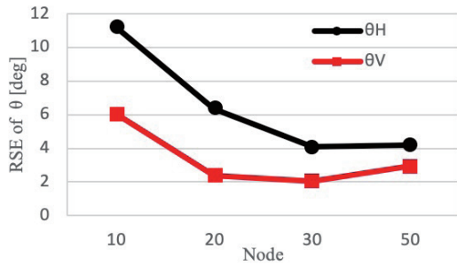
Fig. 4. (Color online) RSE values of angles for different numbers of nodes.
