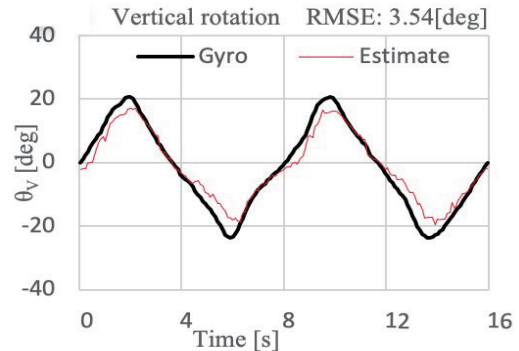
Fig. 14. (Color online) Experimental results of vertical rotation.
