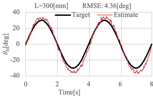
Fig. 9. (Color online) RMSE value of \theta_H obtained using deep learning.
