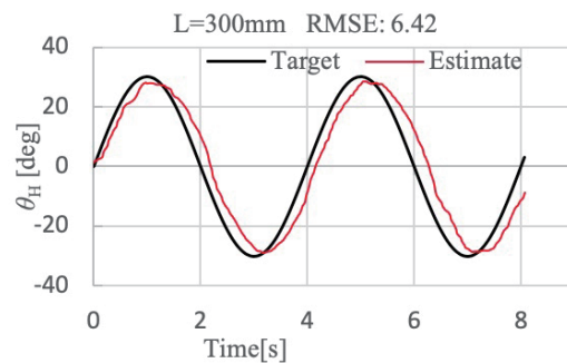
Fig. 10. (Color online) RMSE value of \theta_H obtained by solving PnP problem.
