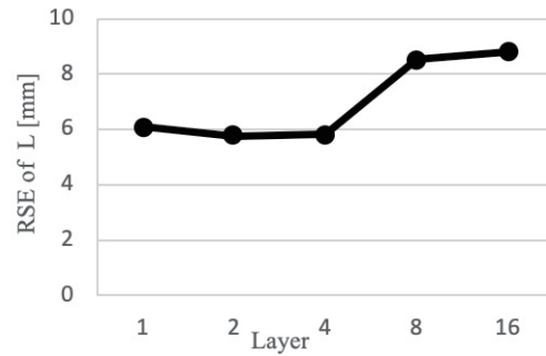
Fig. 7. RSE values of length for different numbers of layers.
