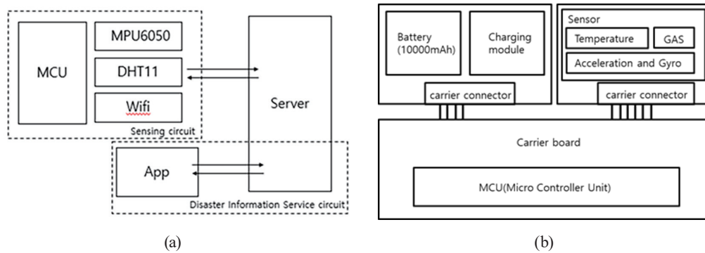
Fig. 4. (a) DISP and (b) CRP configuration diagrams.
