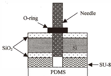
Fig. 4. Schematic of blister test. A needle is inserted into a hole in silicon of known diameter. Nitrogen is allowed to flow and the pressure at which PDMS peels from the SU-8 is recorded.
