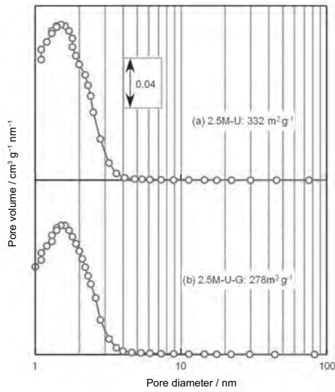
Fig. 8. Pore size distributions of m-SnO 2 powders prepared with UT before aging. (a) Before and (b) after MG.
