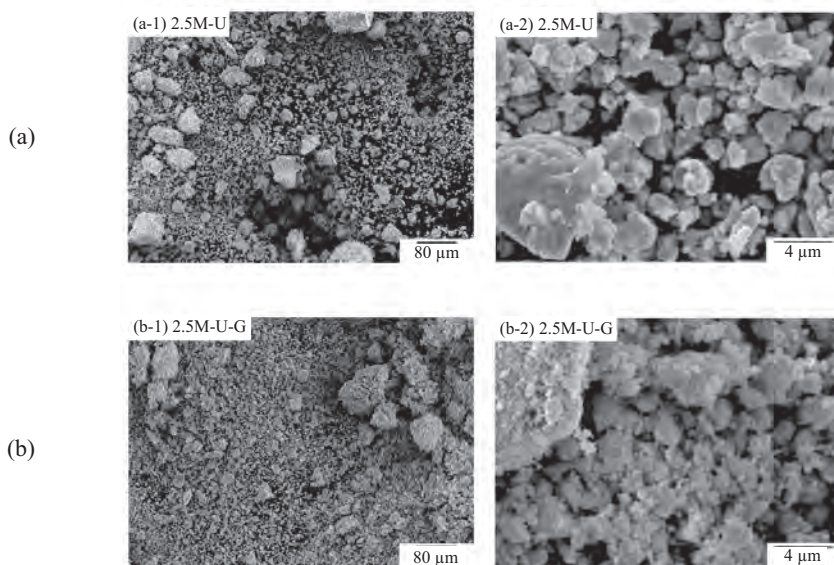
Fig. 7. SEM photographs of m\text{-SnO}_2 powders prepared with UT before aging. (a) Before and (b) after MG.
