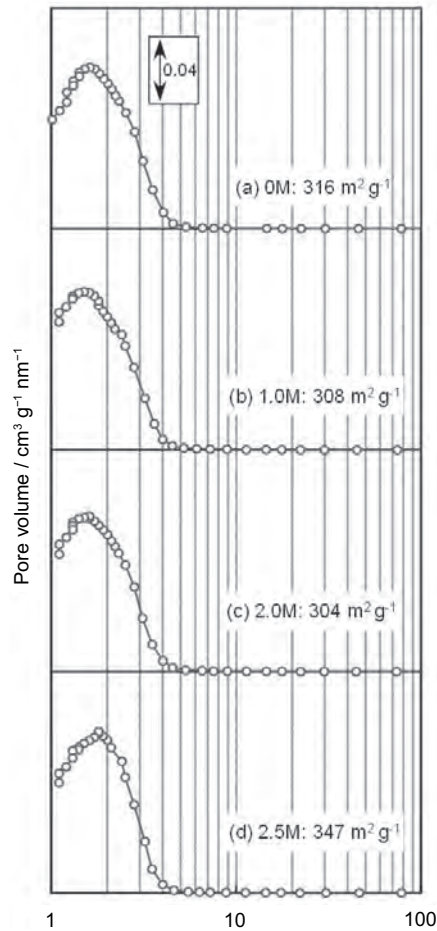
Fig. 2. Pore size distributions of m-SnO 2 powders prepared at various molar ratios of MES/SS. The powders were not subjected to UT or MG.
