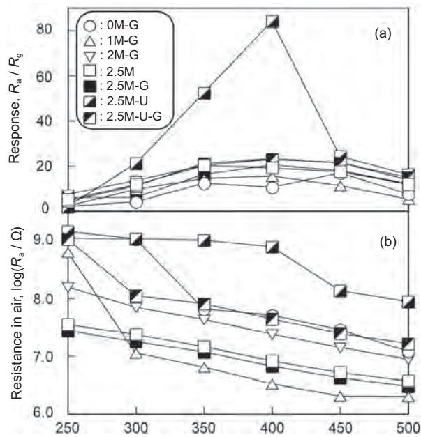
Fig. 9. Operating temperature dependence of (a) response to 1000 ppm H 2 and (b) resistance in air of several m-SnO 2 sensors.
