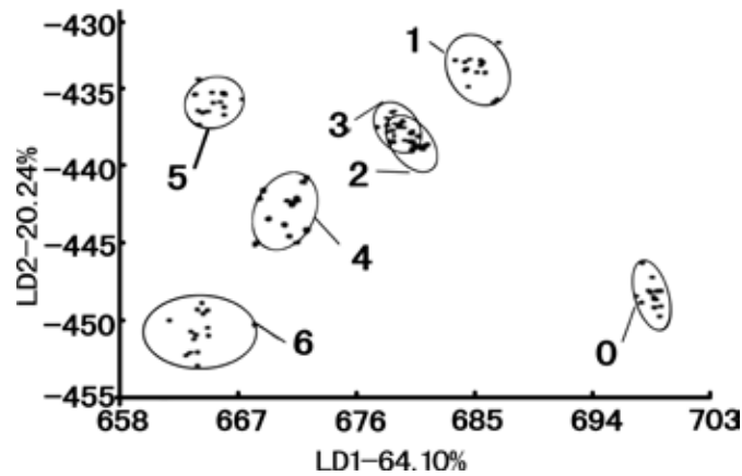
Fig. 4. LDA analysis of meat stored from 0–6 d.
